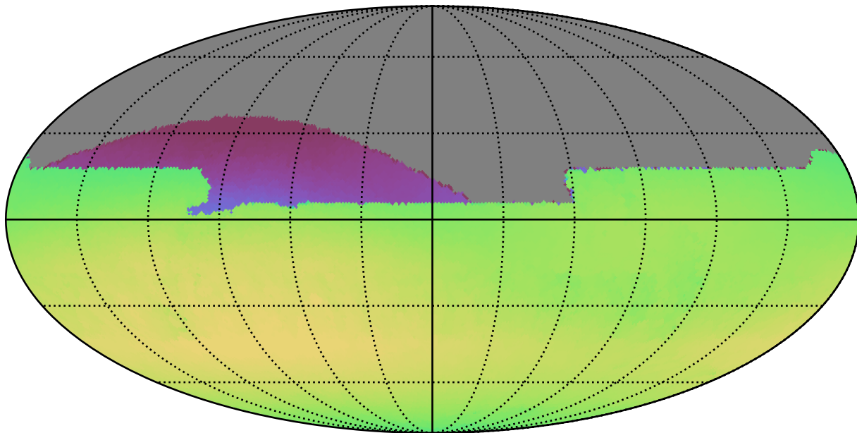
ddf_half_v3.4_10yrs All sky all bands: Max skyBrightness
