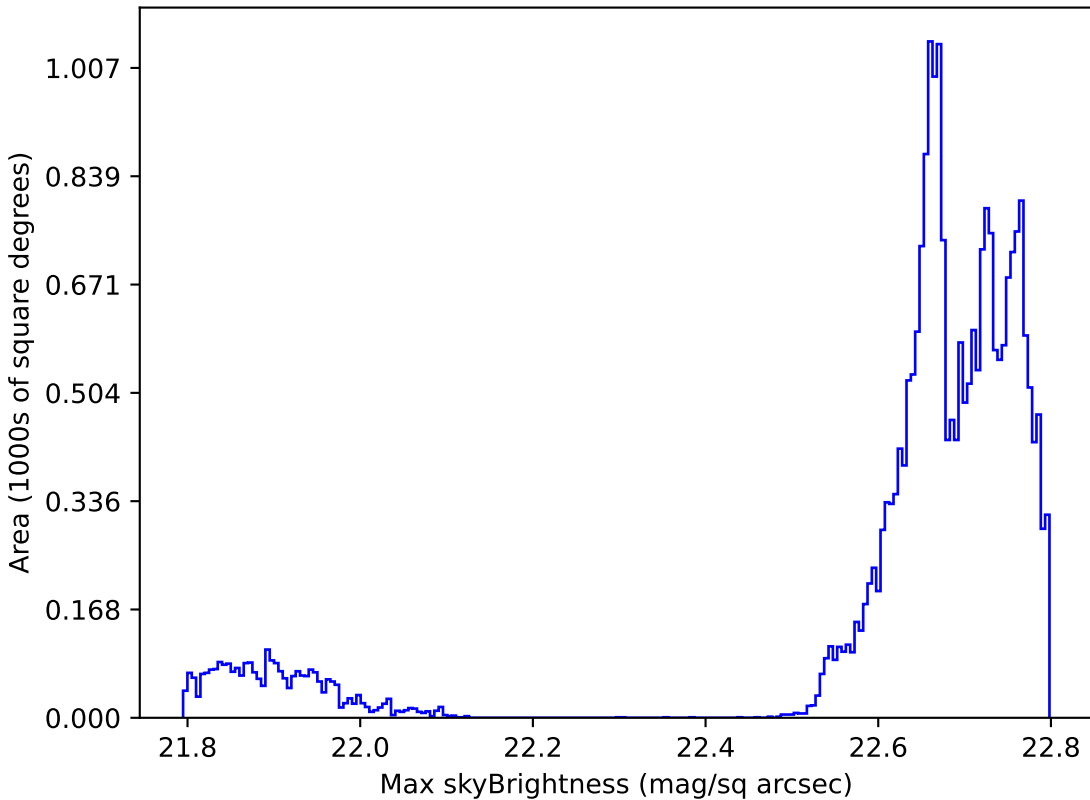
ddf_half_v3.4_10yrs All sky all bands: Max skyBrightness
