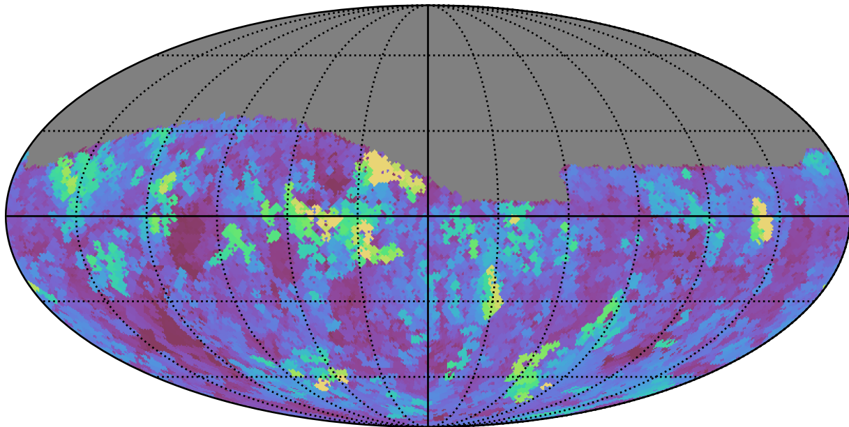
ddf_half_v3.4_10yrs Yr 1 z band: Max seeingGeom
