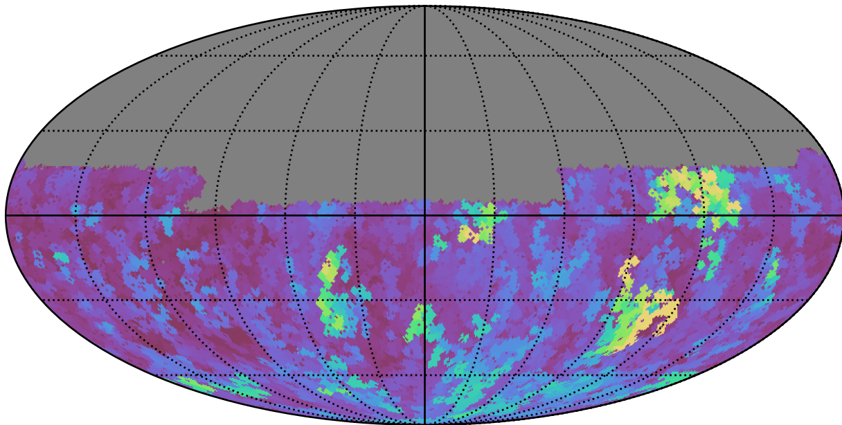
ddf_half_v3.4_10yrs Yr 1 u band: Max seeingGeom
