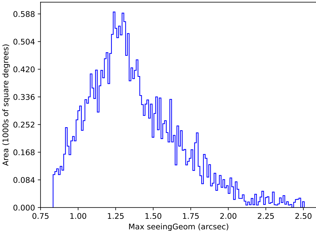
ddf_half_v3.4_10yrs Yr 1 r band: Max seeingGeom
