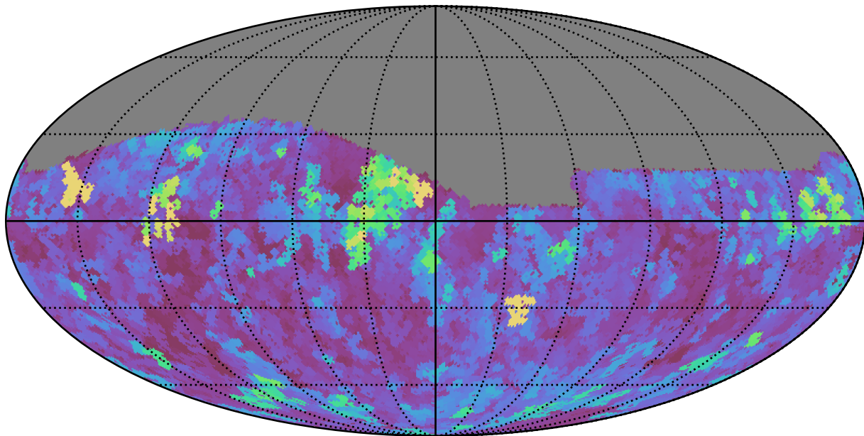
ddf_half_v3.4_10yrs Yr 1 i band: Max seeingGeom
