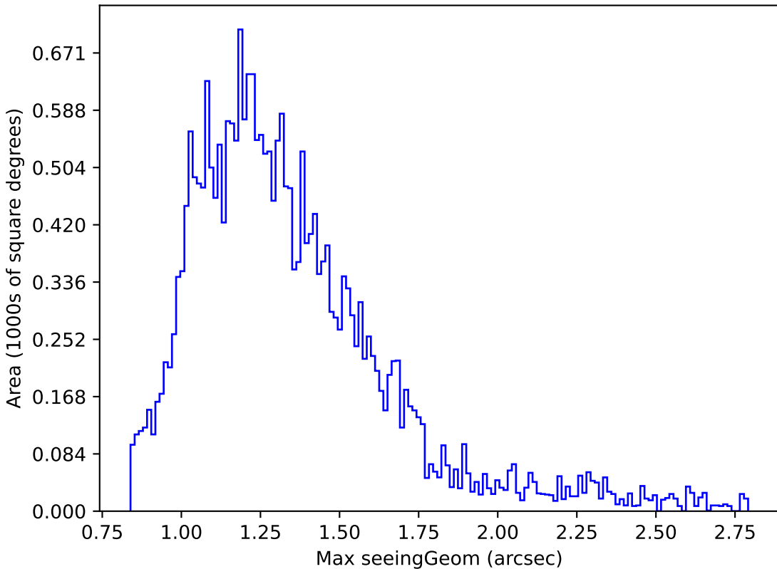
ddf_half_v3.4_10yrs Yr 1 i band: Max seeingGeom
