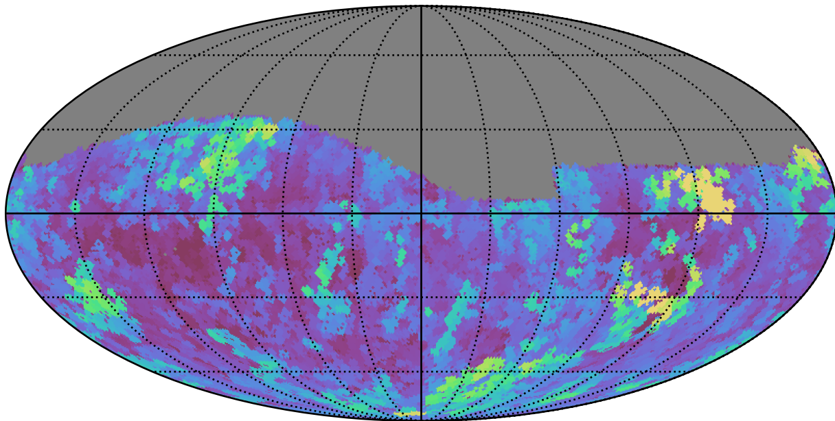
ddf_half_v3.4_10yrs Yr 1 g band: Max seeingGeom
