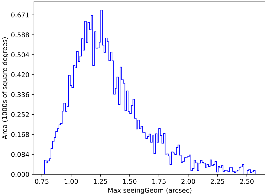
ddf_half_v3.4_10yrs Yr 1 g band: Max seeingGeom
