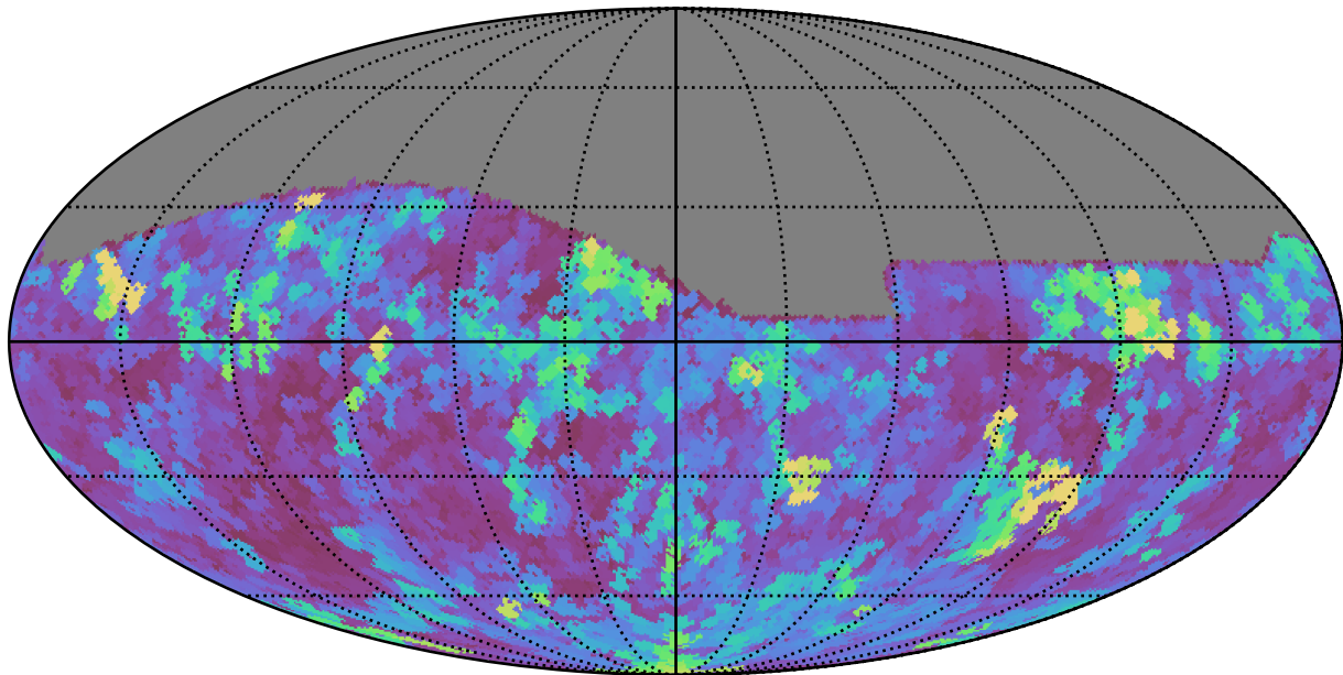
ddf_half_v3.4_10yrs Yr 1 all bands: Max seeingGeom
