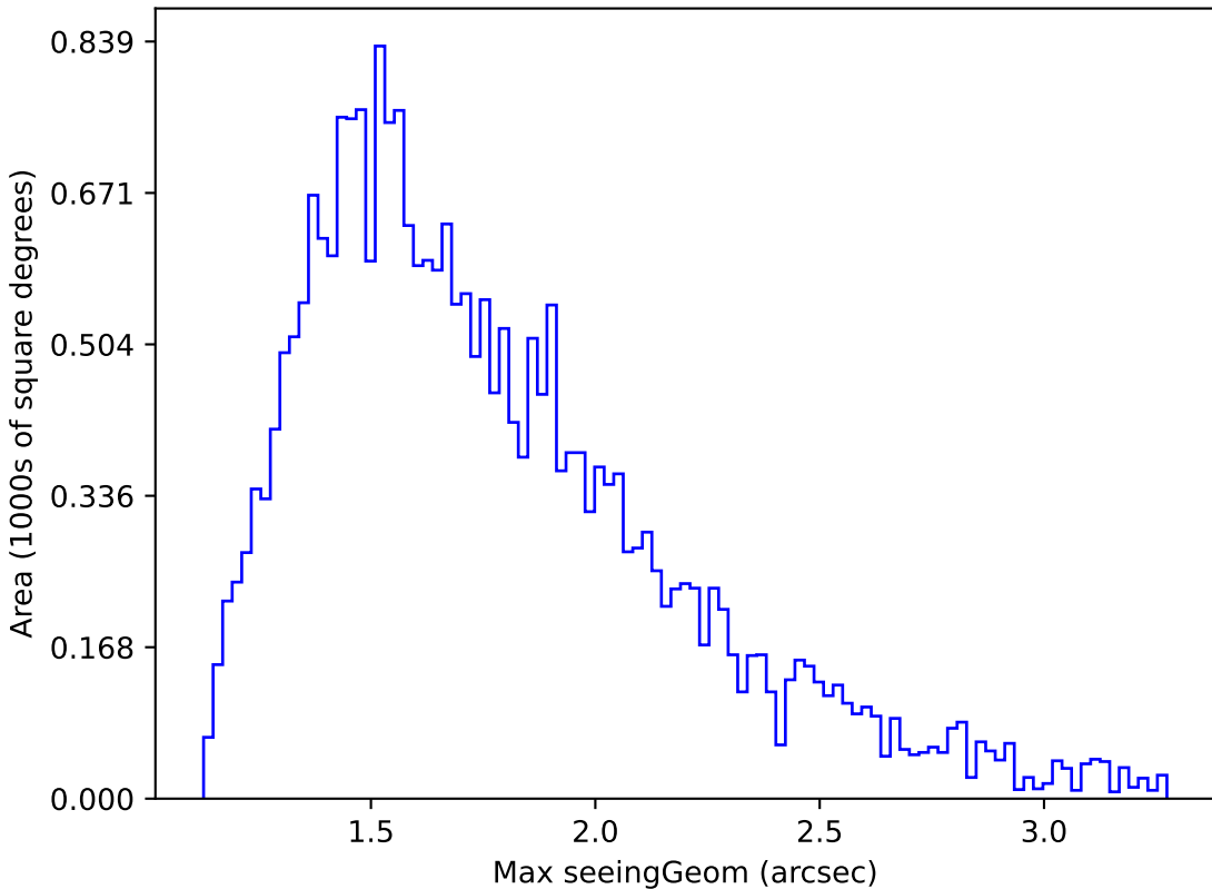
ddf_half_v3.4_10yrs Yr 1 all bands: Max seeingGeom
