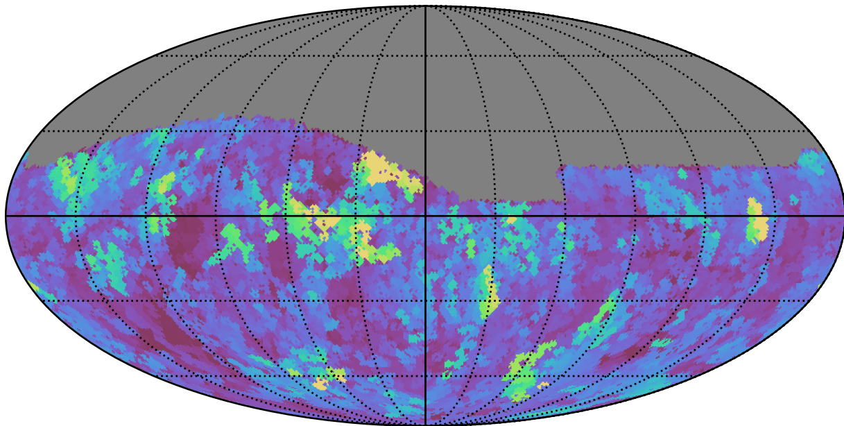
ddf_half_v3.4_10yrs Yr 1 z band: Max seeingEff
