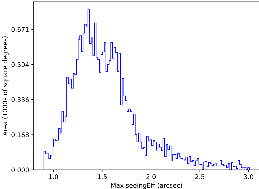
ddf_half_v3.4_10yrs Yr 1 z band: Max seeingEff
