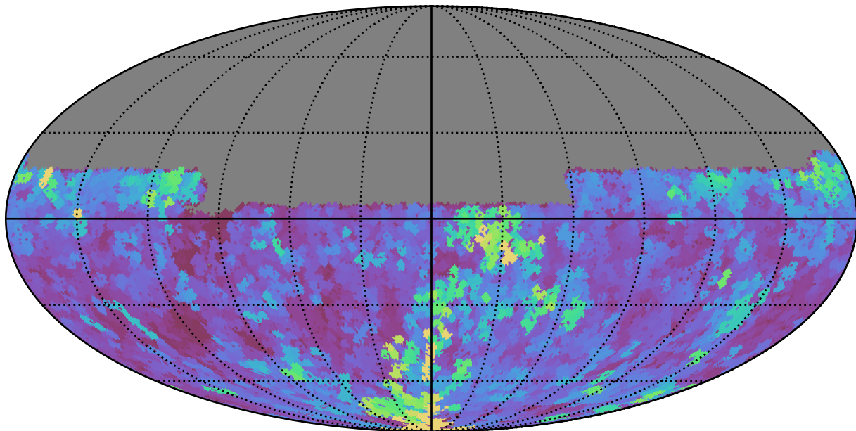
ddf_half_v3.4_10yrs Yr 1 y band: Max seeingEff
