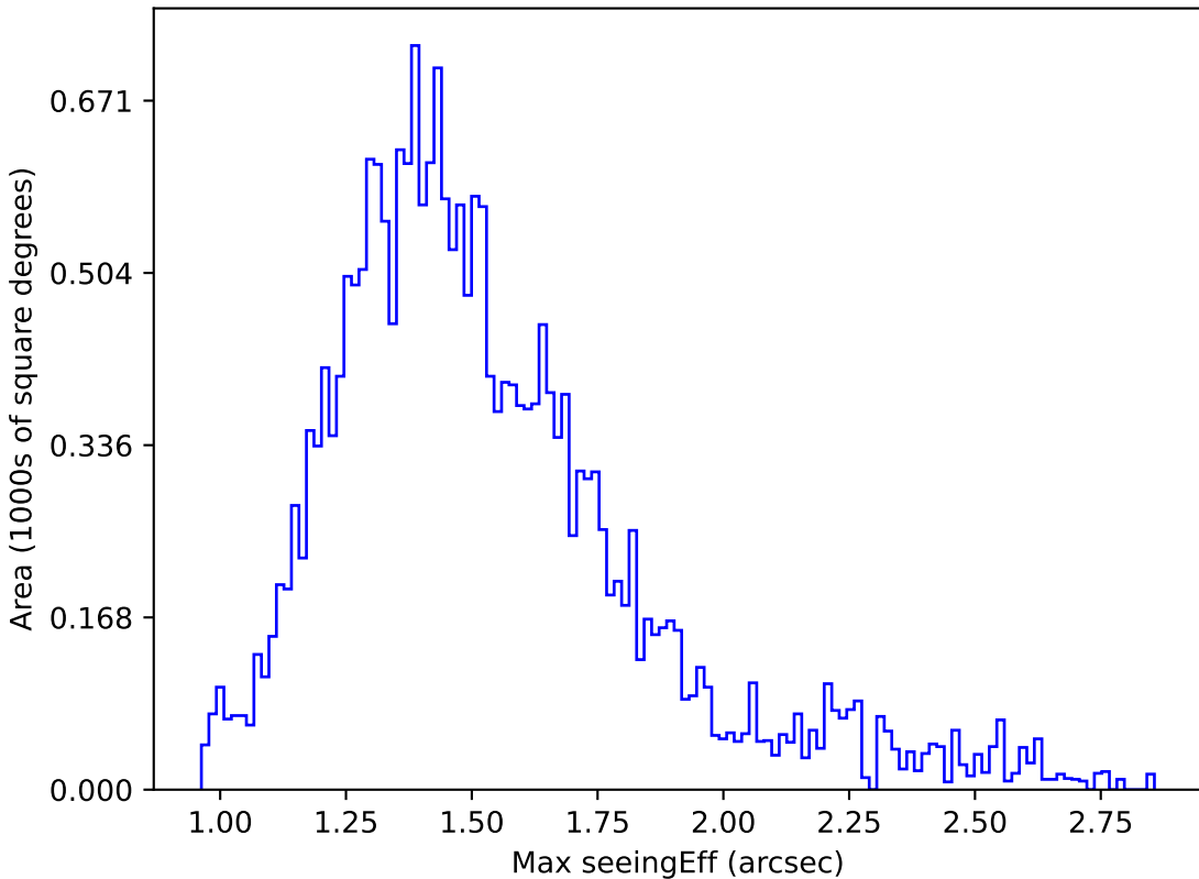
ddf_half_v3.4_10yrs Yr 1 y band: Max seeingEff
