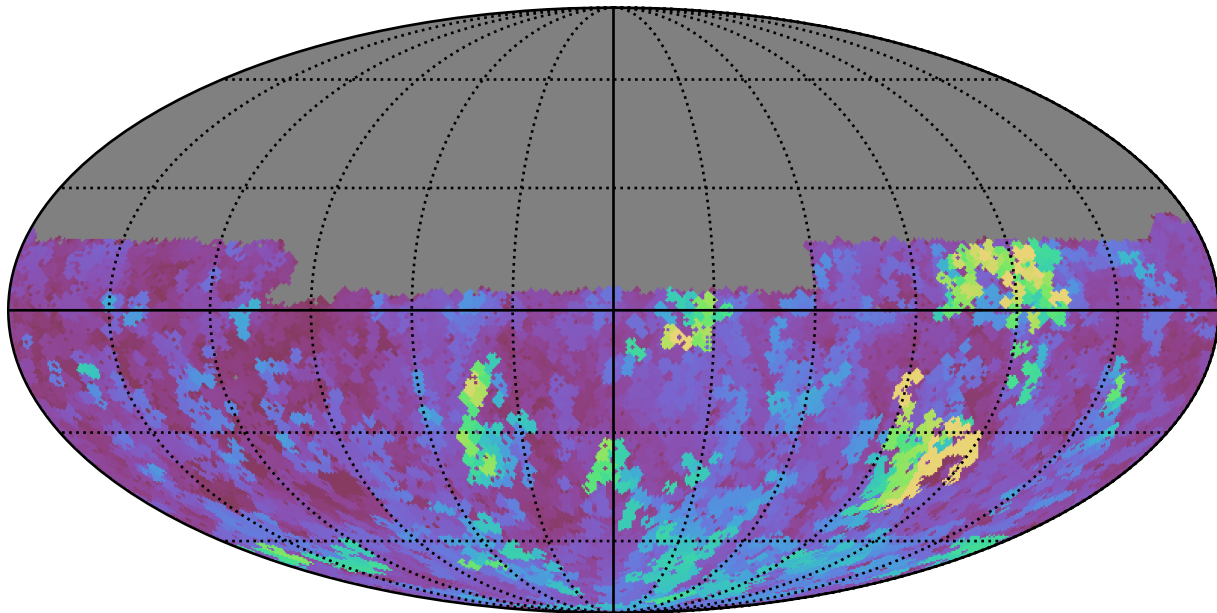
ddf_half_v3.4_10yrs Yr 1 u band: Max seeingEff
