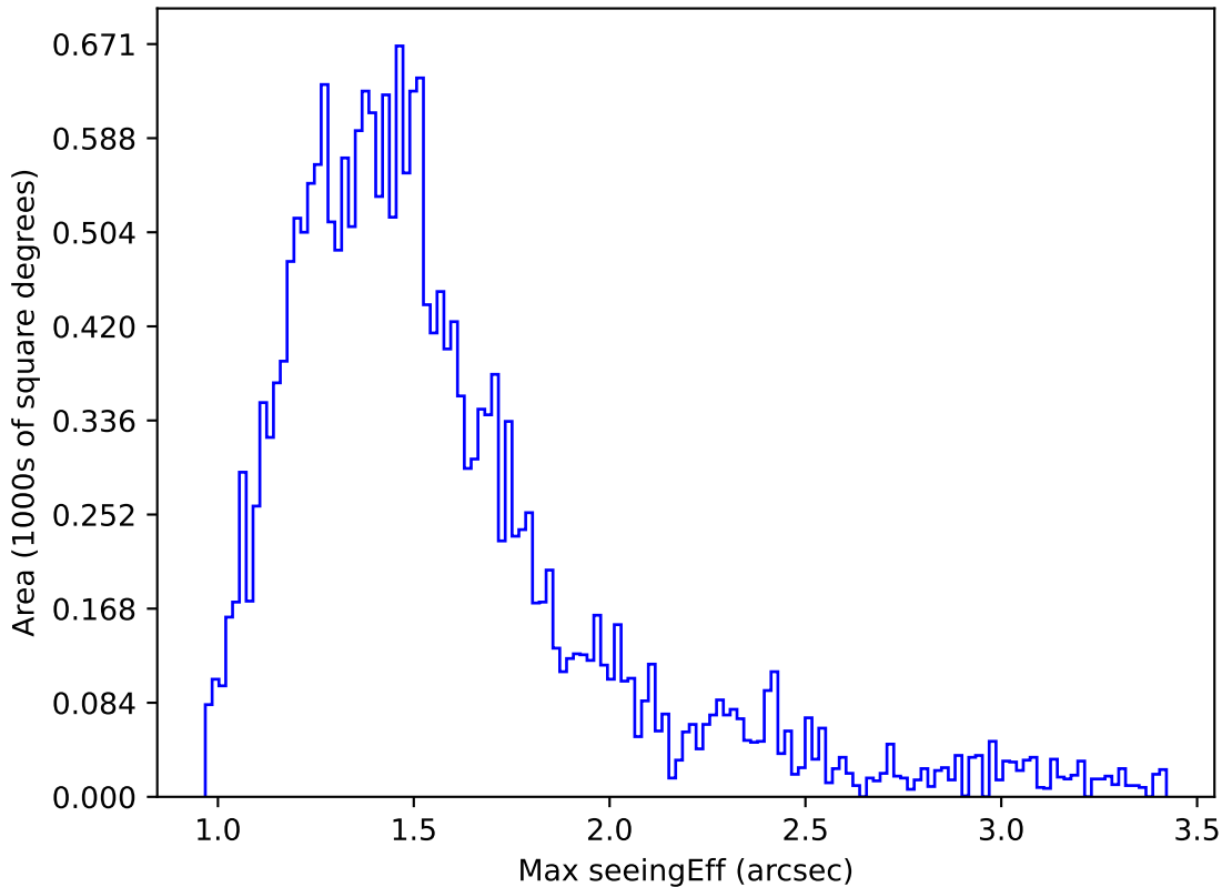
ddf_half_v3.4_10yrs Yr 1 u band: Max seeingEff
