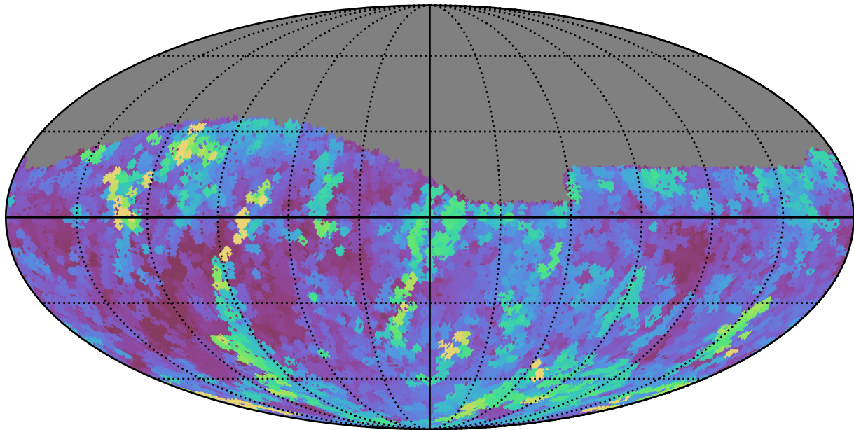
ddf_half_v3.4_10yrs Yr 1 r band: Max seeingEff
