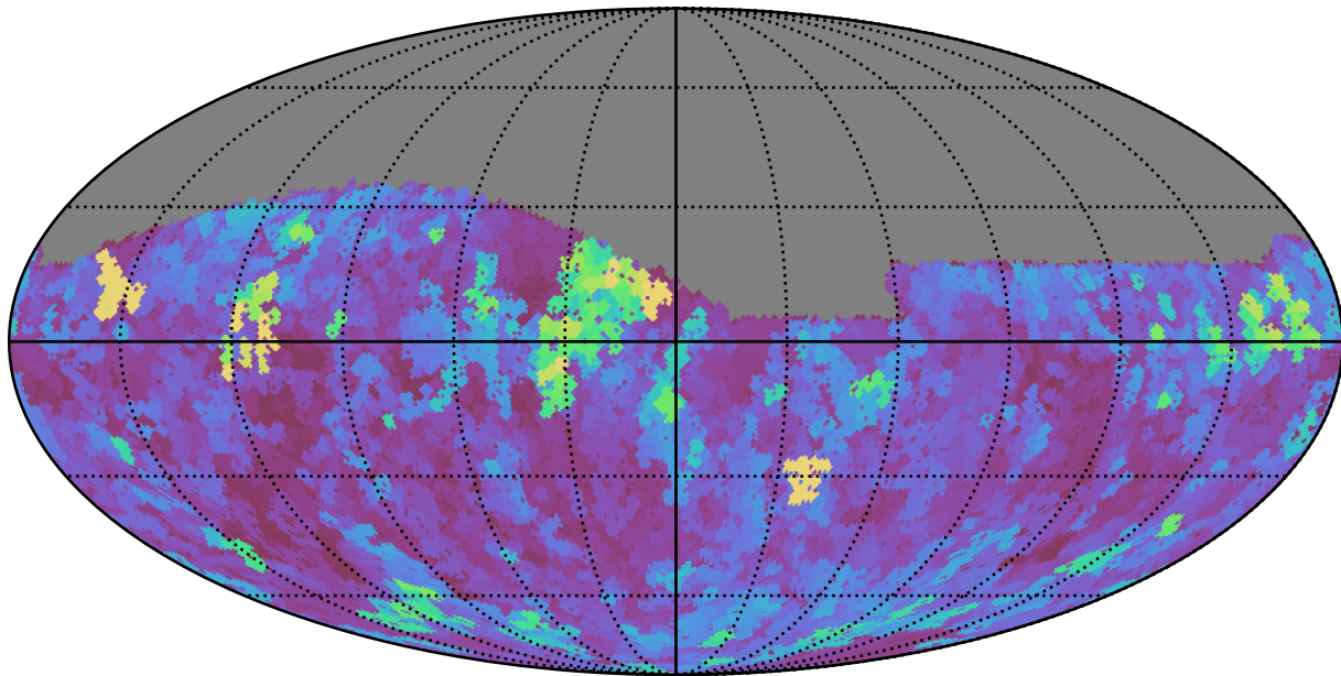
ddf_half_v3.4_10yrs Yr 1 i band: Max seeingEff
