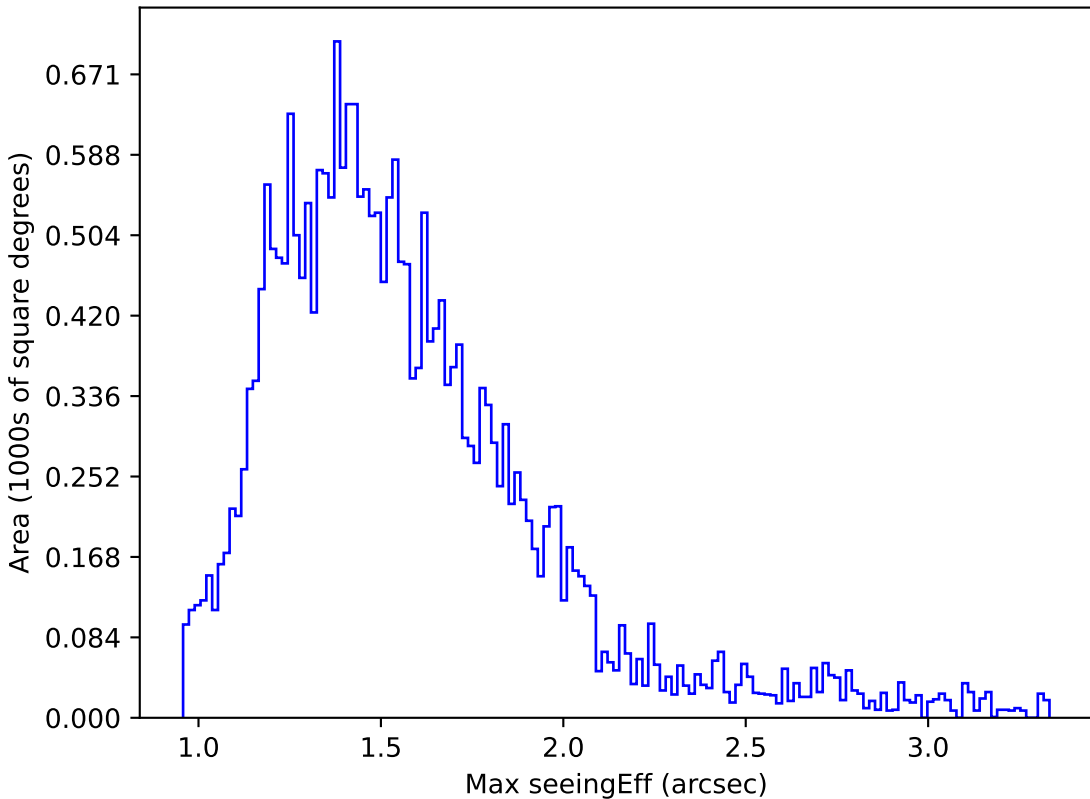
ddf_half_v3.4_10yrs Yr 1 i band: Max seeingEff
