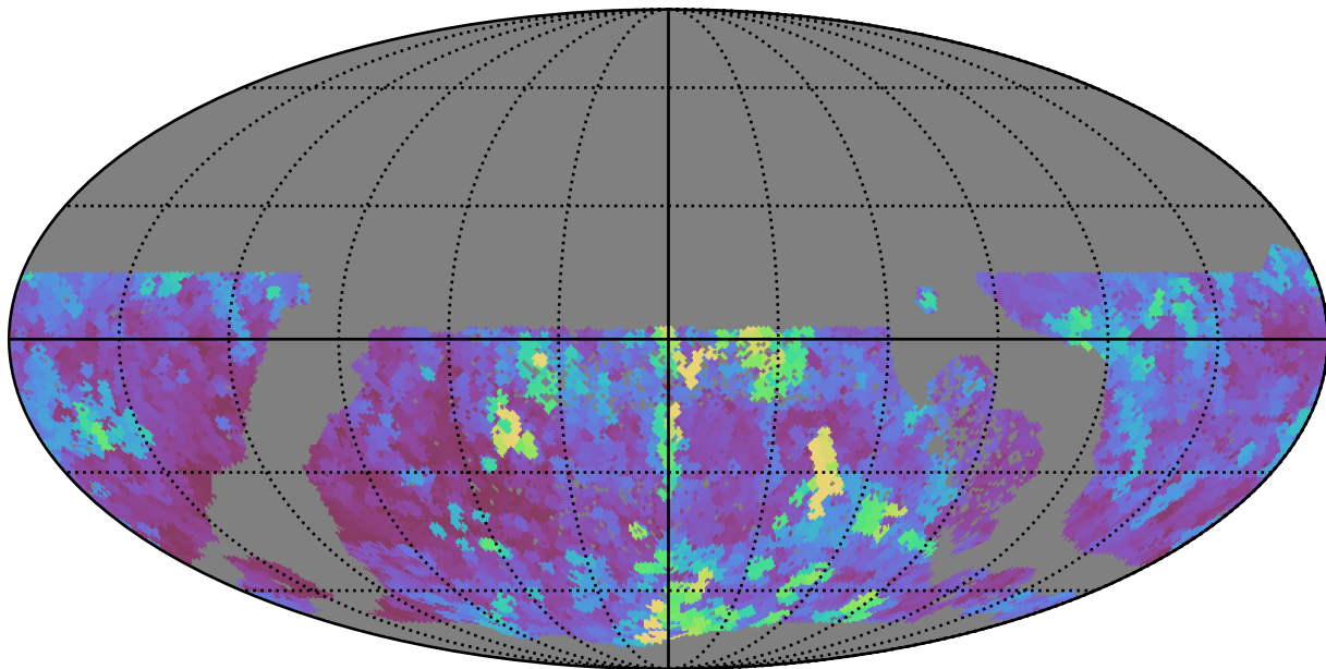
ddf_half_v3.4_10yrs WFD z band: Max seeingEff
