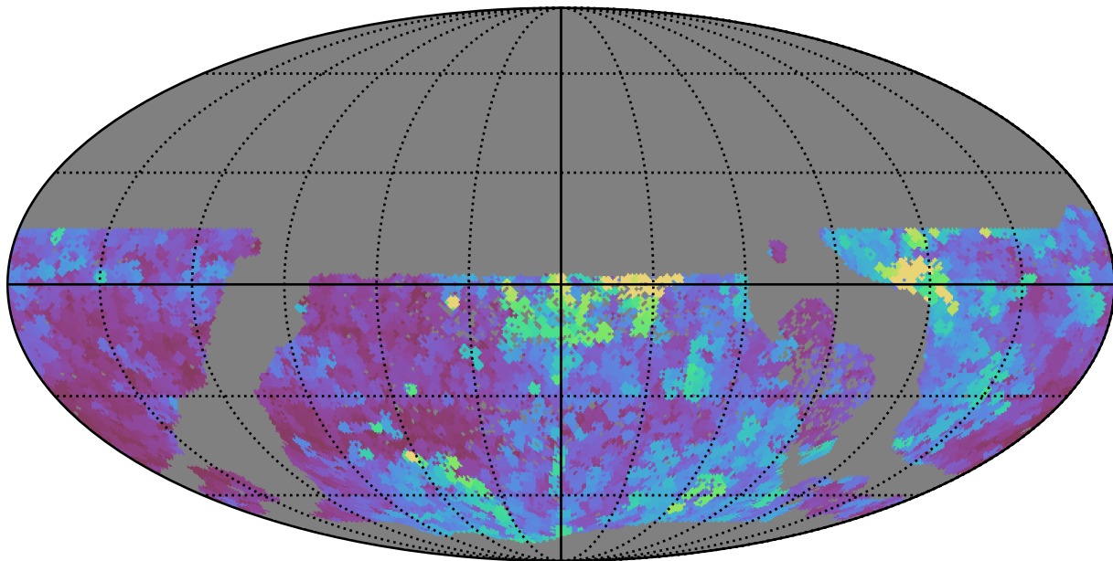
ddf_half_v3.4_10yrs WFD y band: Max seeingEff
