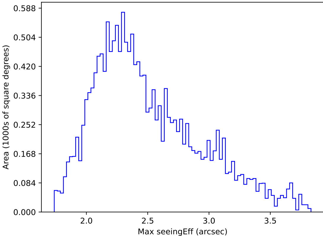
ddf_half_v3.4_10yrs WFD u band: Max seeingEff
