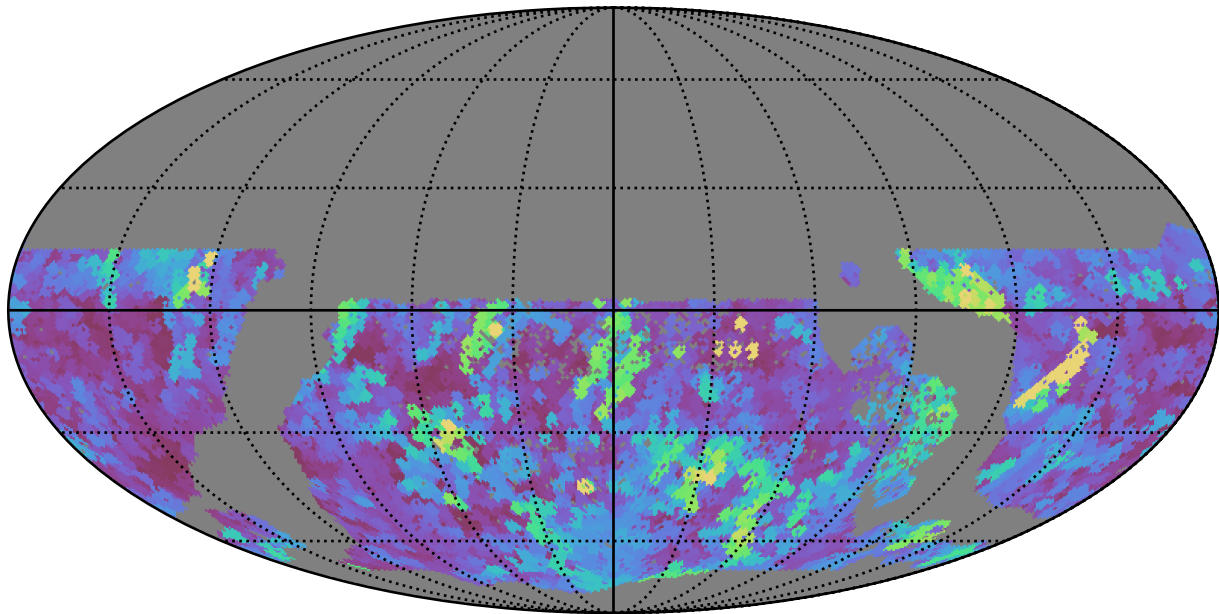
ddf_half_v3.4_10yrs WFD r band: Max seeingEff
