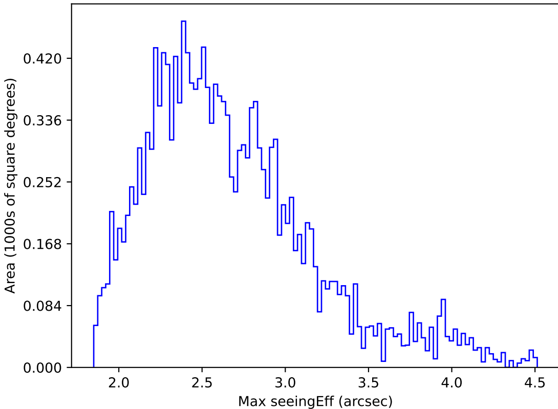
ddf_half_v3.4_10yrs WFD r band: Max seeingEff
