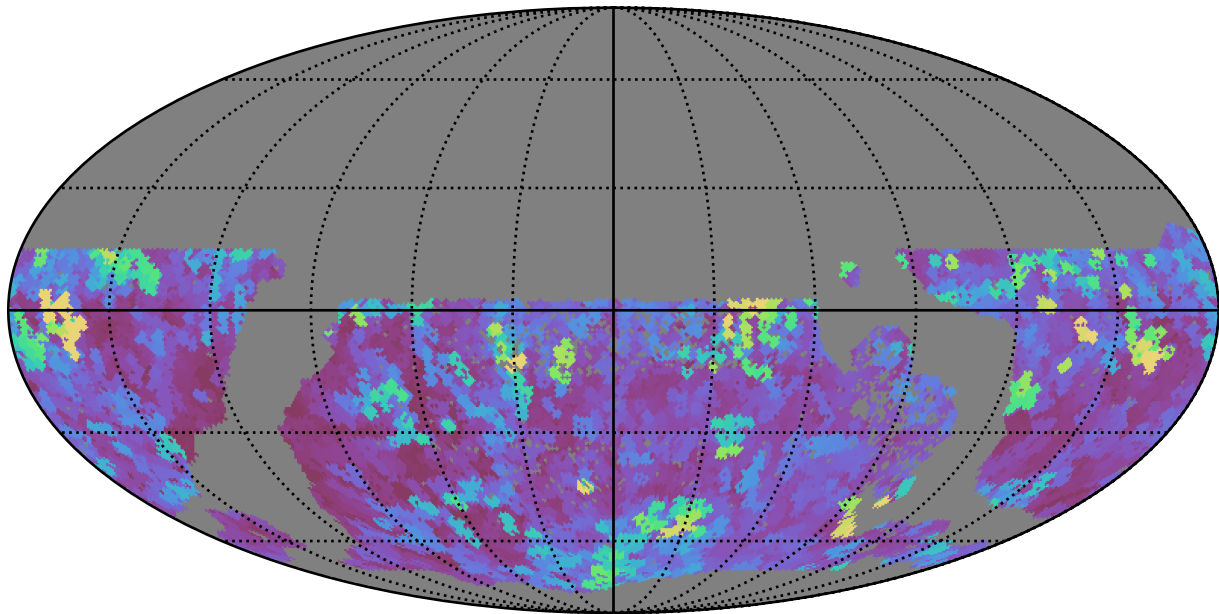
ddf_half_v3.4_10yrs WFD i band: Max seeingEff
