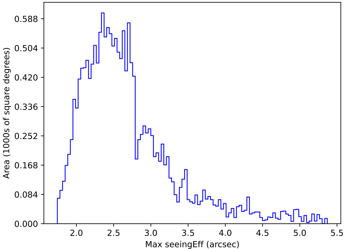
ddf_half_v3.4_10yrs WFD i band: Max seeingEff
