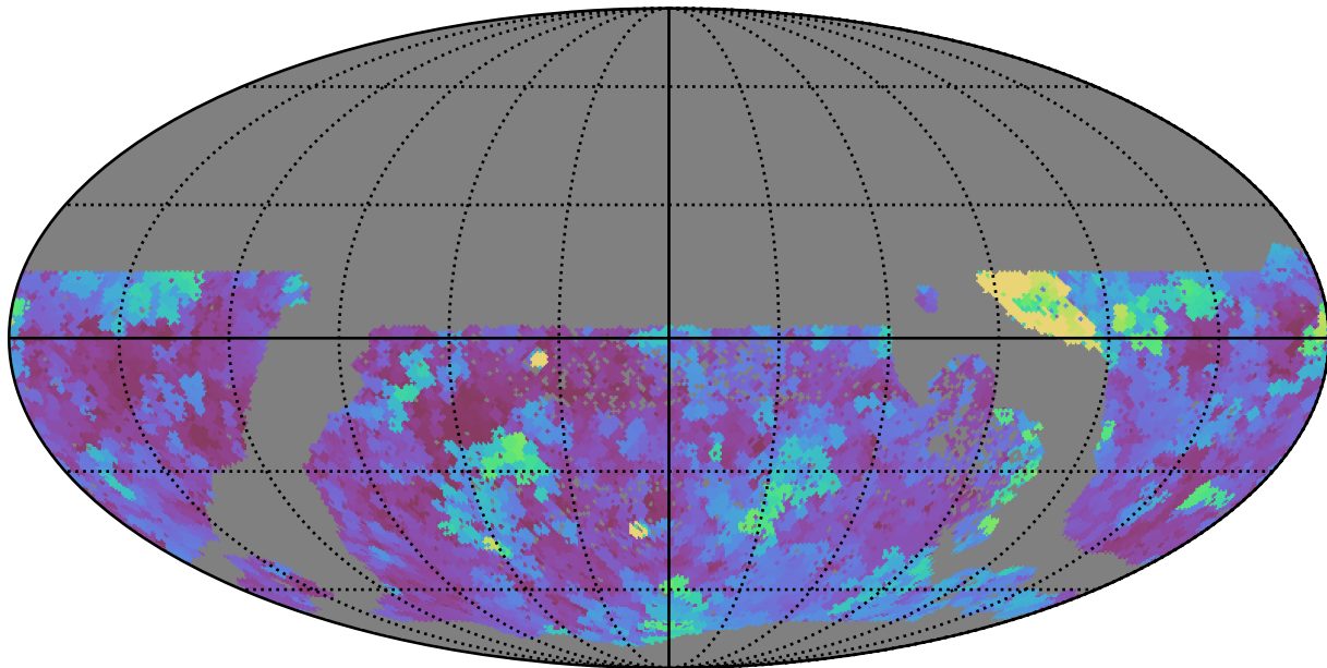
ddf_half_v3.4_10yrs WFD g band: Max seeingEff
