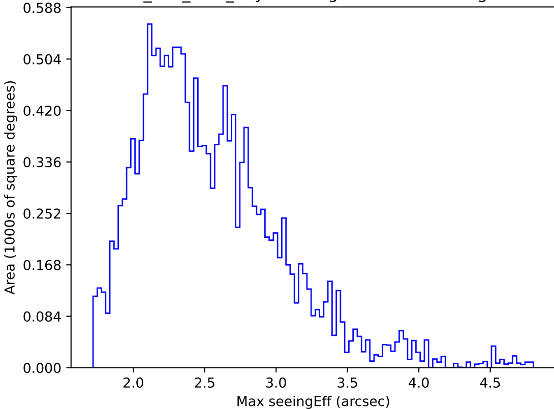
ddf_half_v3.4_10yrs WFD g band: Max seeingEff
