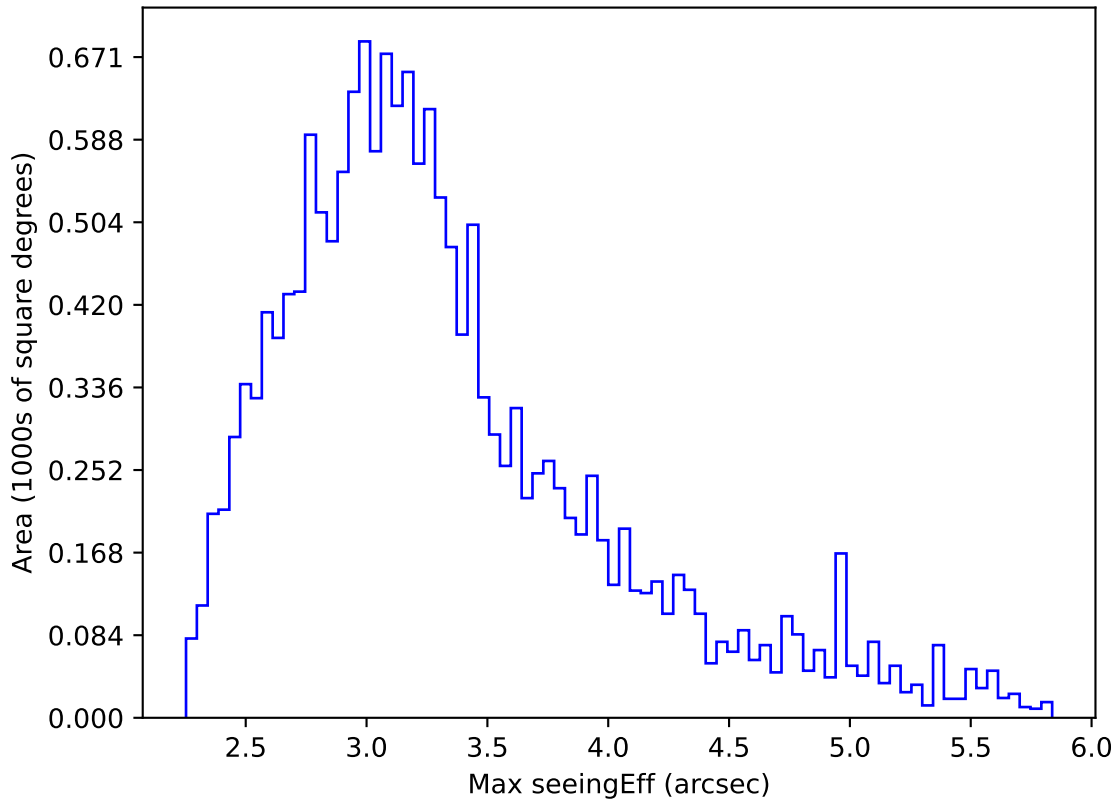
ddf_half_v3.4_10yrs WFD all bands: Max seeingEff
