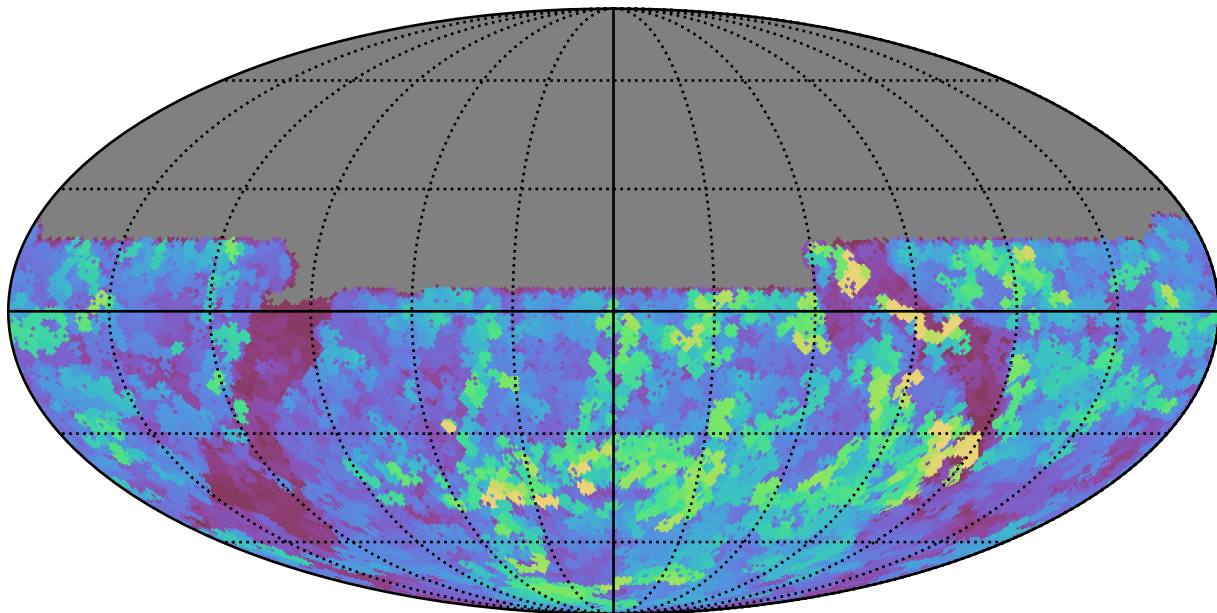
ddf_half_v3.4_10yrs All sky u band: Max seeingEff
