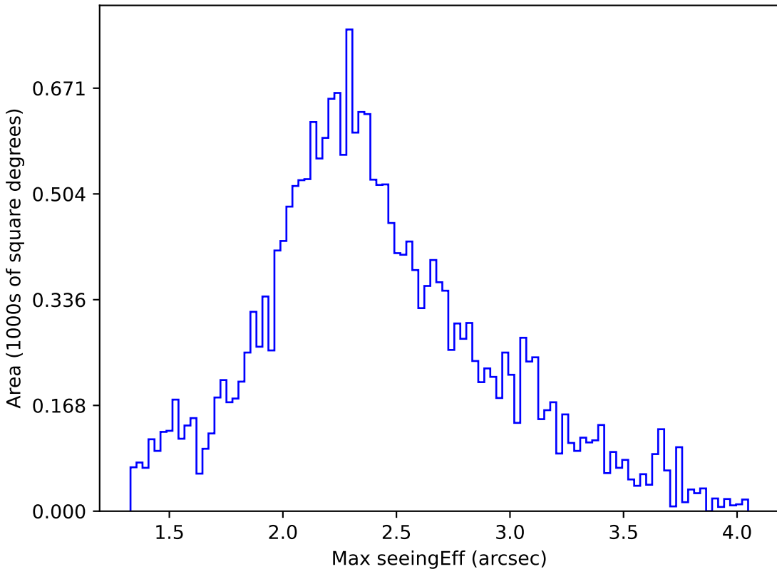
ddf_half_v3.4_10yrs All sky u band: Max seeingEff
