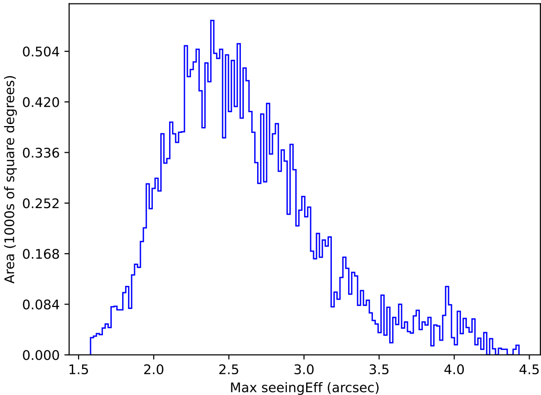
ddf_half_v3.4_10yrs All sky r band: Max seeingEff
