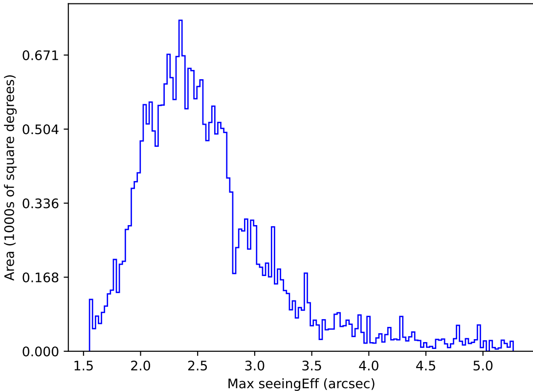
ddf_half_v3.4_10yrs All sky i band: Max seeingEff
