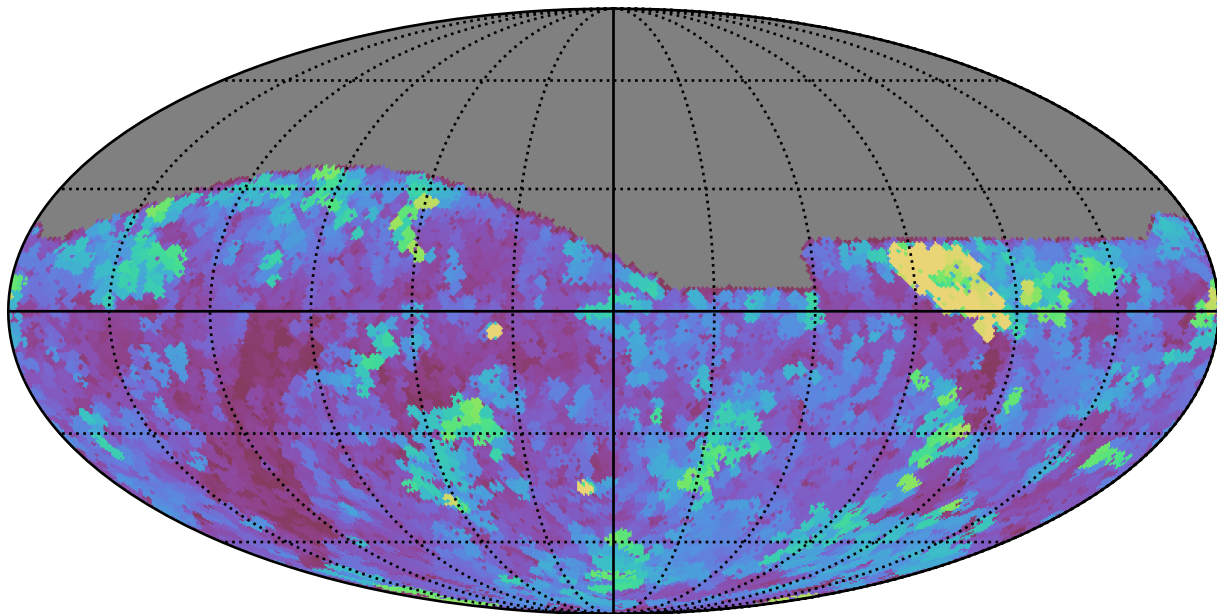
ddf_half_v3.4_10yrs All sky g band: Max seeingEff
