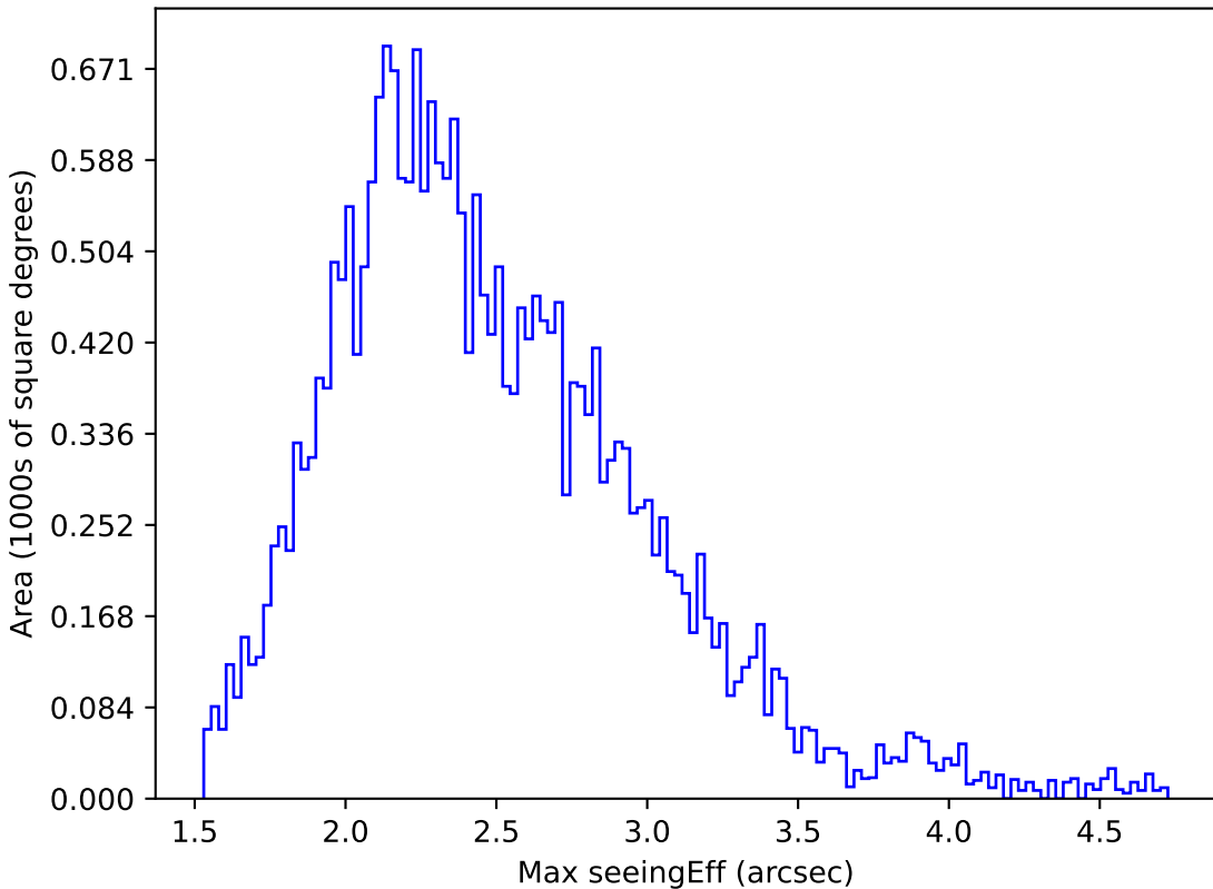
ddf_half_v3.4_10yrs All sky g band: Max seeingEff
