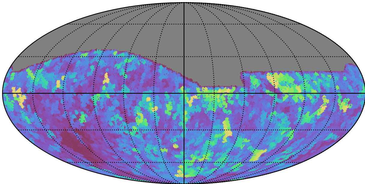
ddf_half_v3.4_10yrs All sky all bands: Max seeingEff
