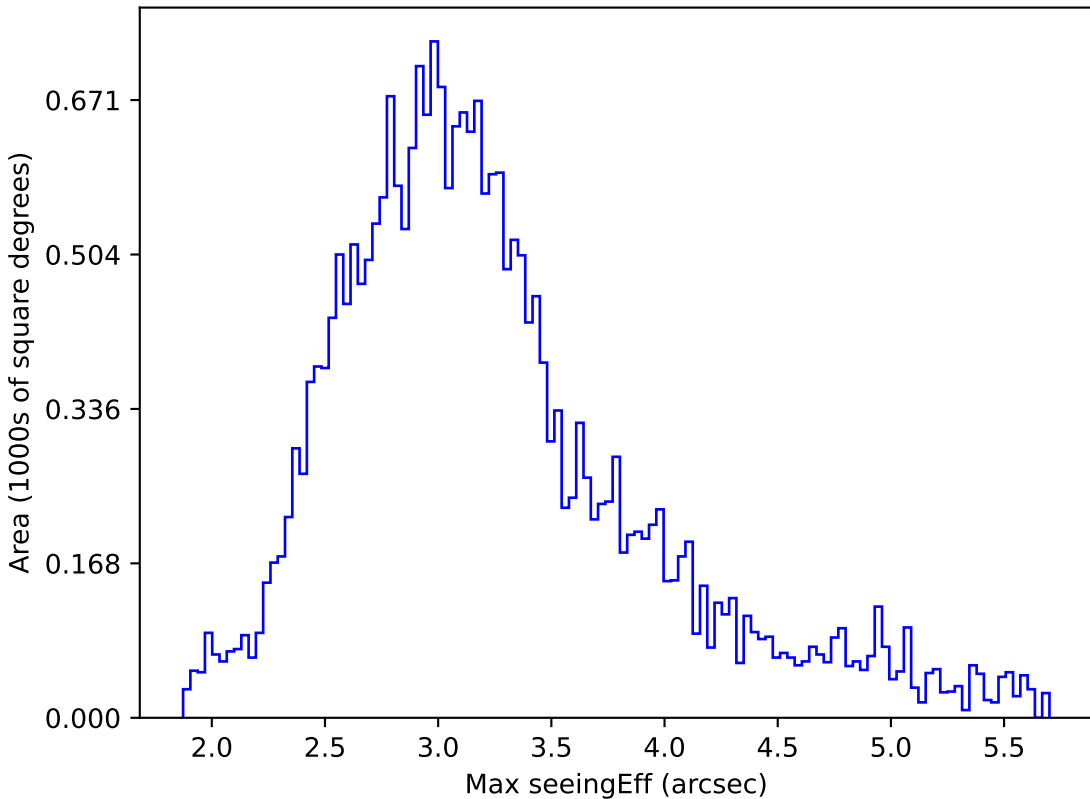
ddf_half_v3.4_10yrs All sky all bands: Max seeingEff
