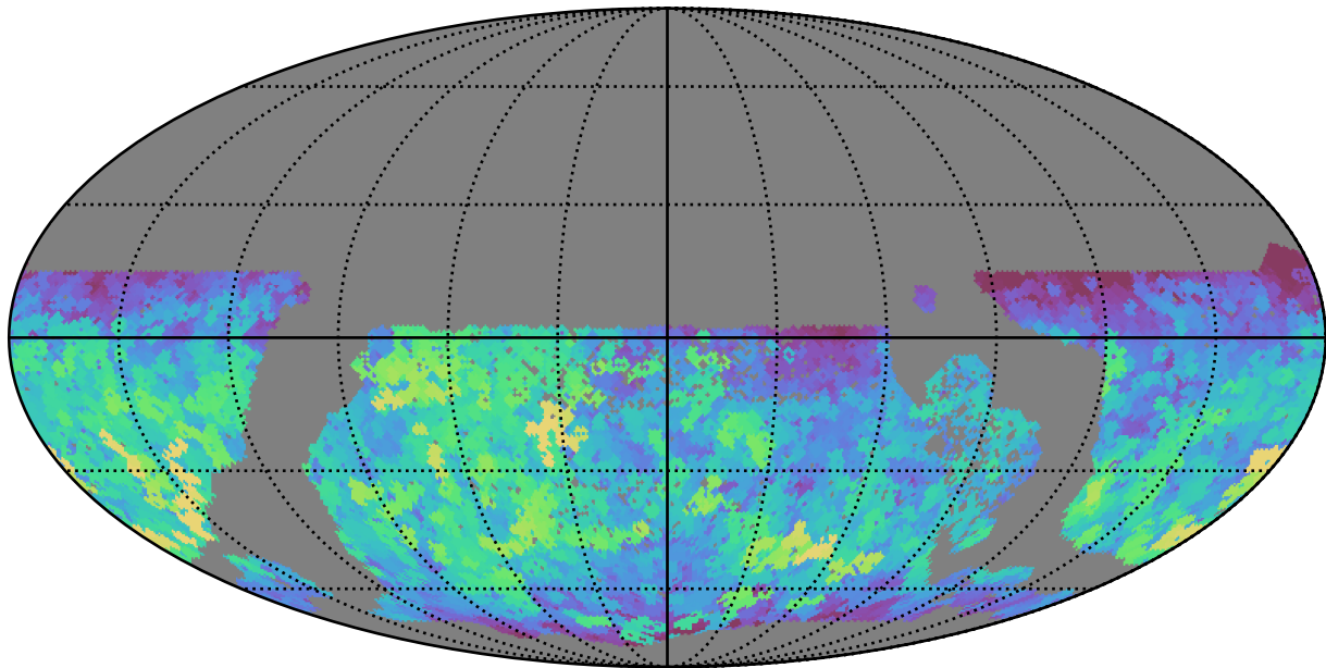
ddf_half_v3.4_10yrs WFD z band: Max saturation_mag
