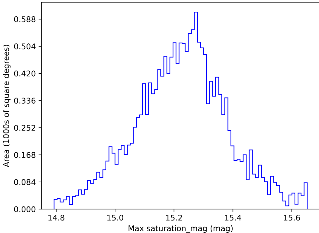
ddf_half_v3.4_10yrs WFD z band: Max saturation_mag
