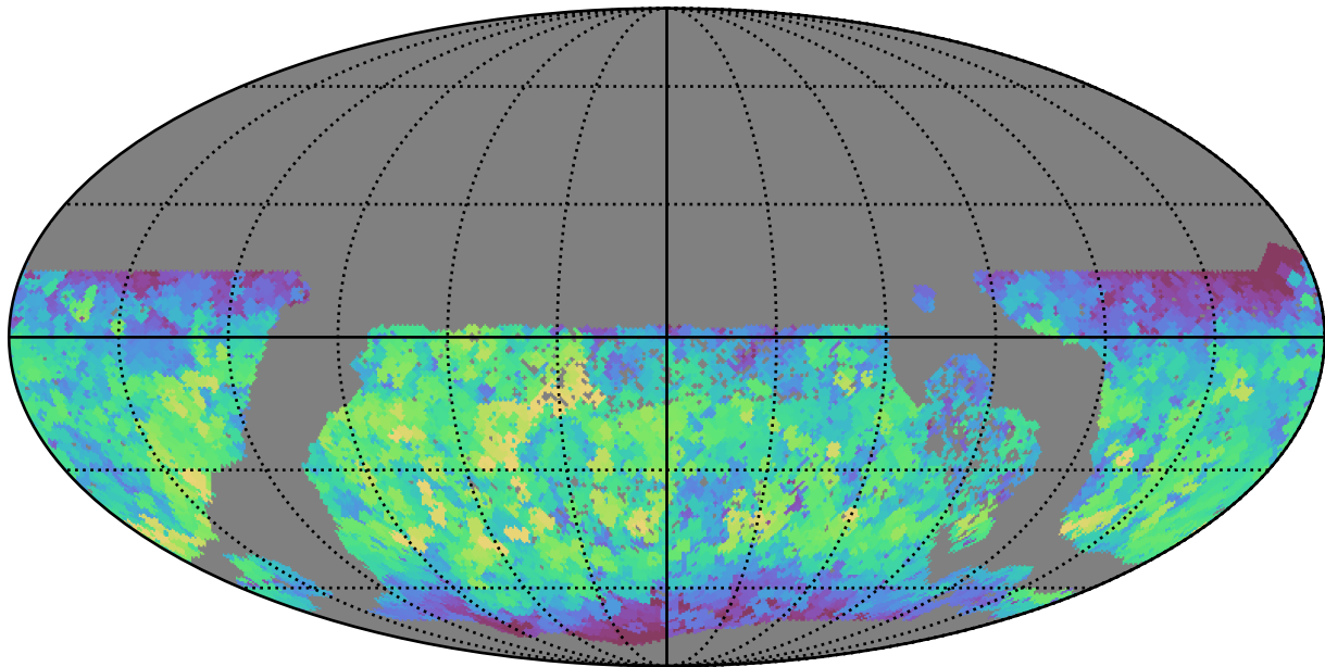
ddf_half_v3.4_10yrs WFD y band: Max saturation_mag
