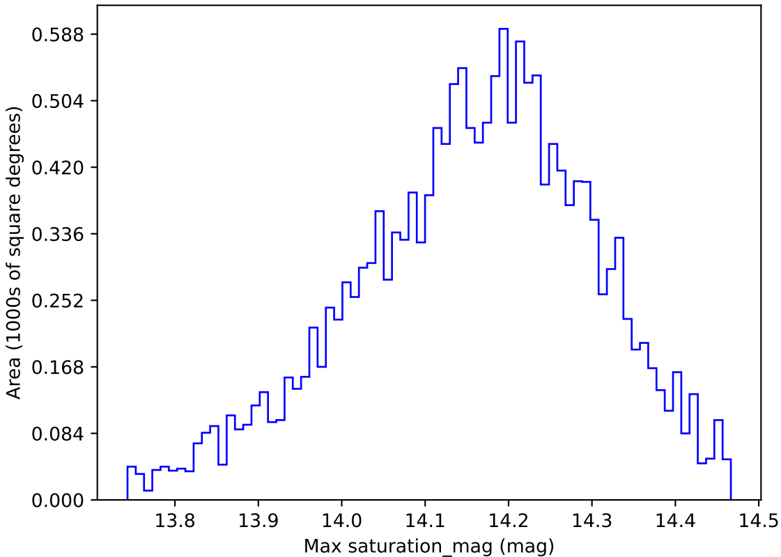
ddf_half_v3.4_10yrs WFD y band: Max saturation_mag
