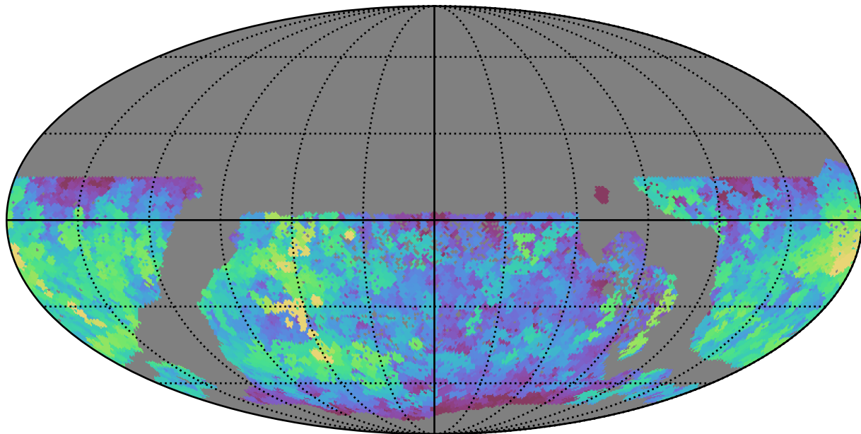
ddf_half_v3.4_10yrs WFD u band: Max saturation_mag
