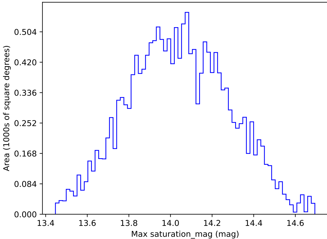
ddf_half_v3.4_10yrs WFD u band: Max saturation_mag
