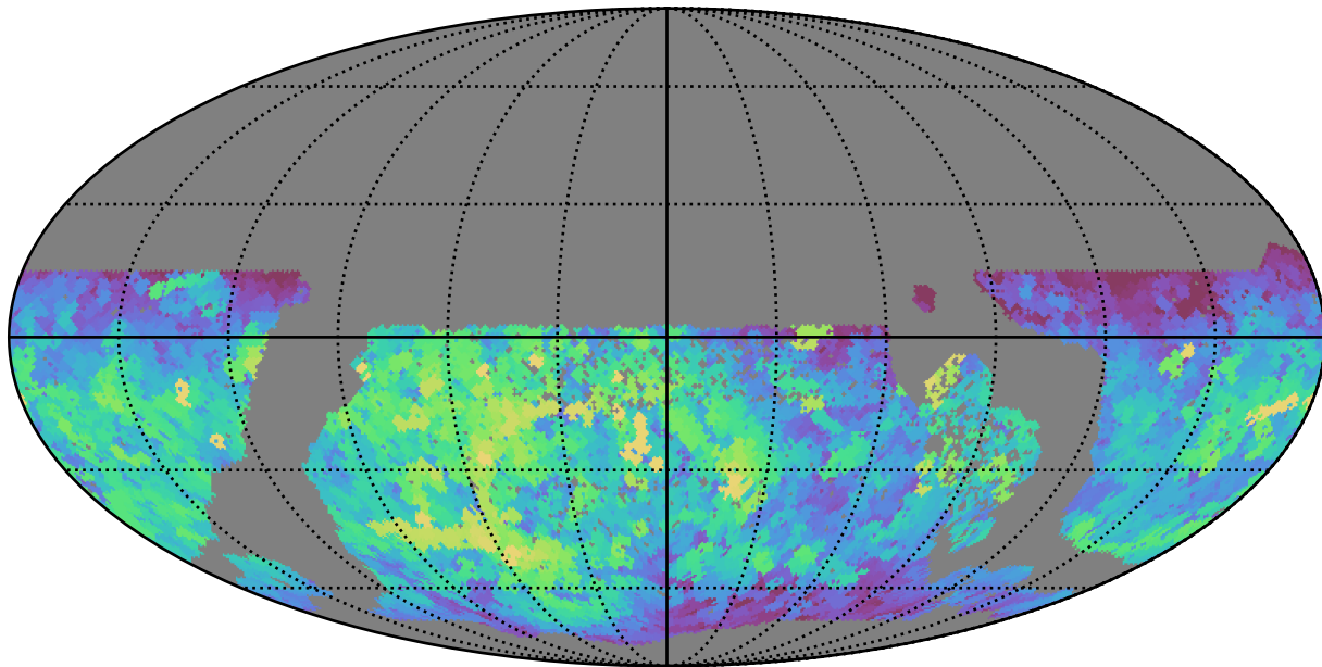
ddf_half_v3.4_10yrs WFD r band: Max saturation_mag
