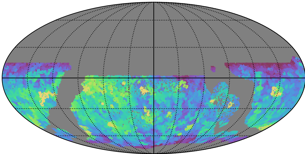
ddf_half_v3.4_10yrs WFD i band: Max saturation_mag
