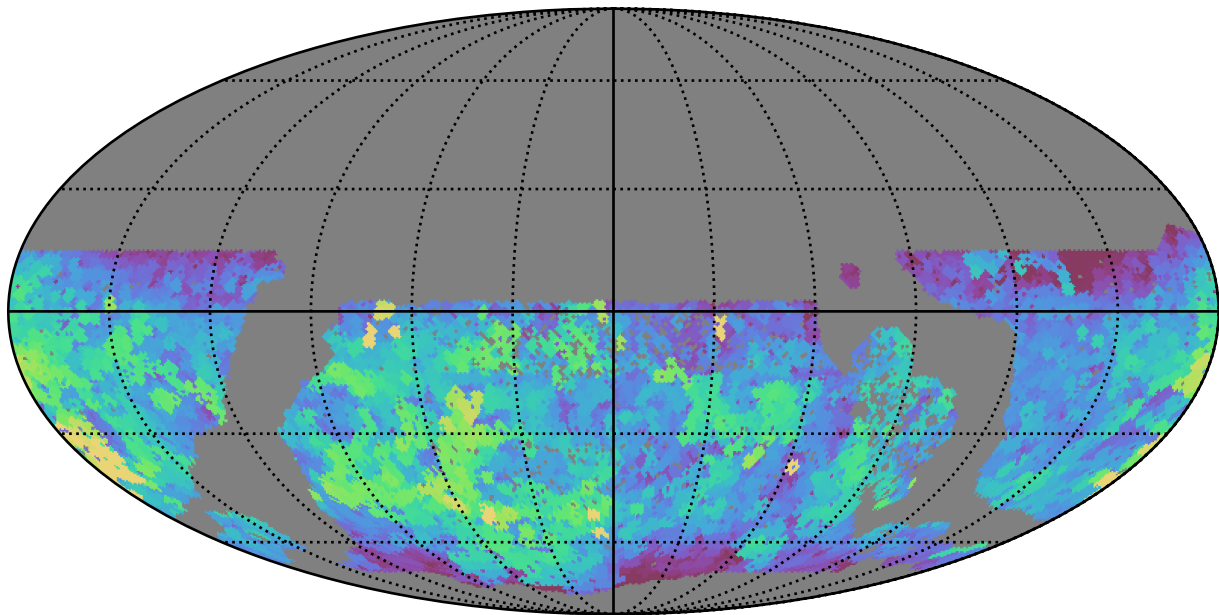
ddf_half_v3.4_10yrs WFD g band: Max saturation_mag
