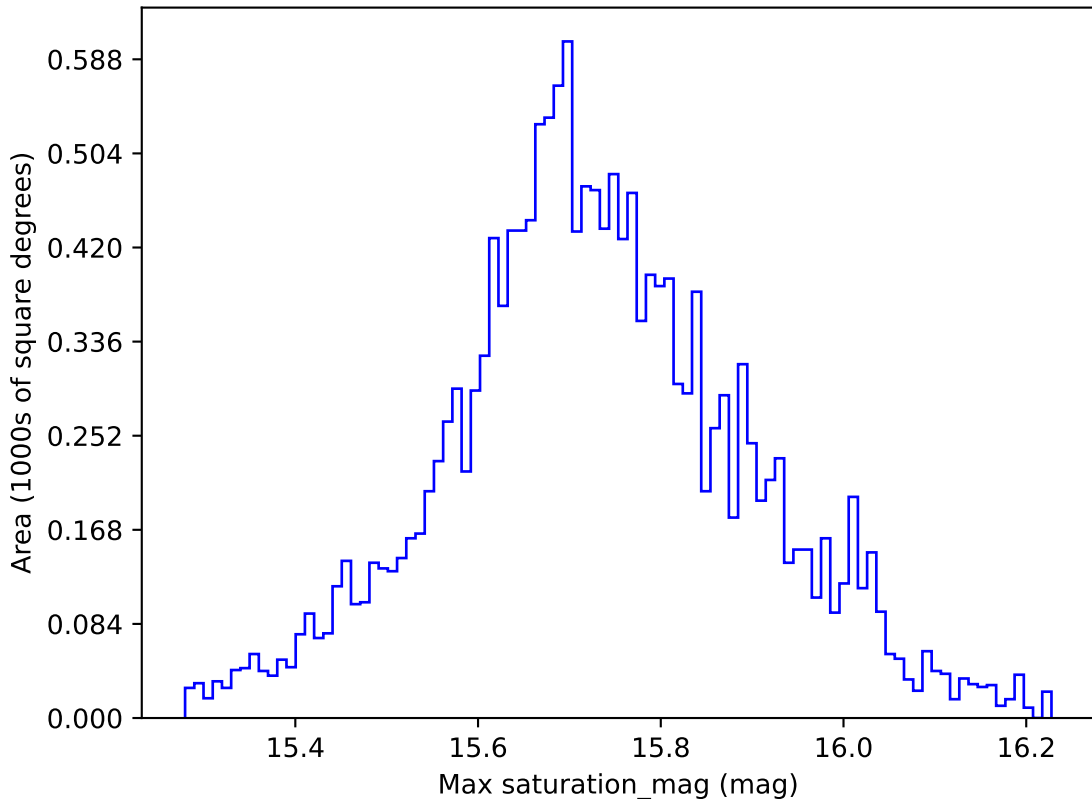
ddf_half_v3.4_10yrs WFD g band: Max saturation_mag
