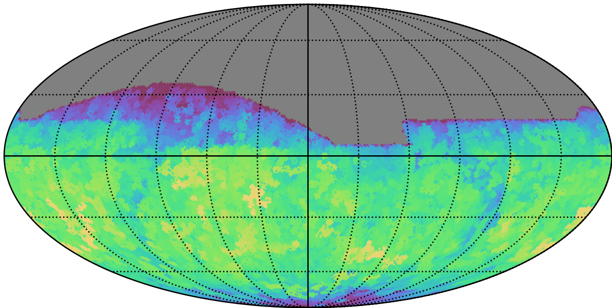
ddf_half_v3.4_10yrs All sky z band: Max saturation_mag
