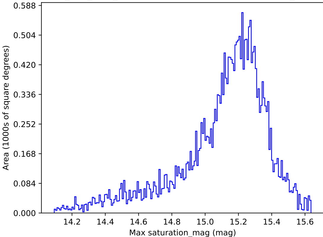
ddf_half_v3.4_10yrs All sky z band: Max saturation_mag
